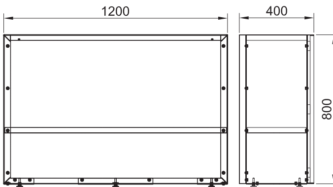
Deco Planter 120x40x80 cm
