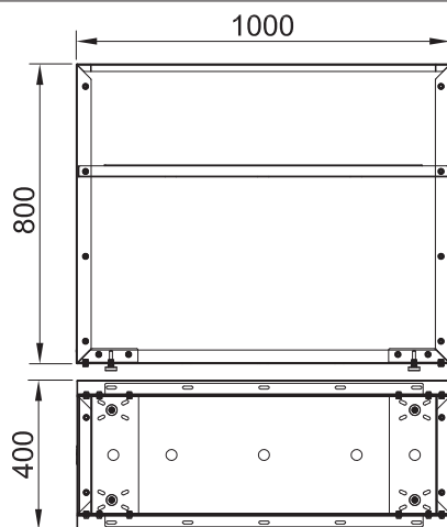
Metal Planter Corten for 100x40x80 cm
